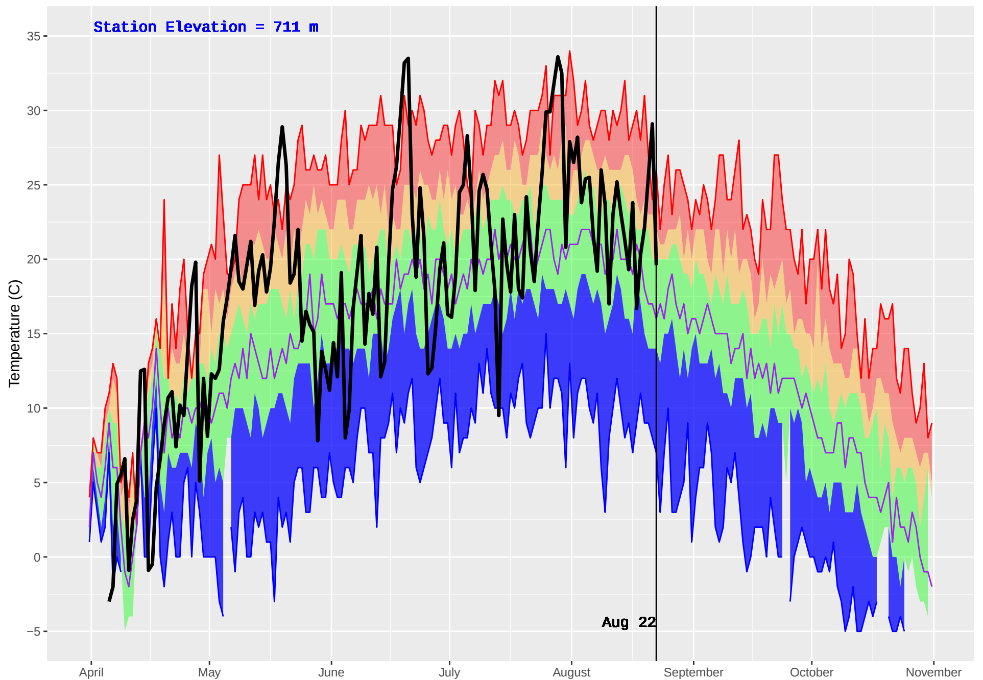
TOAD RIVER (126) : Historical (1981–2016) and Current (2018) Daily Temperature
